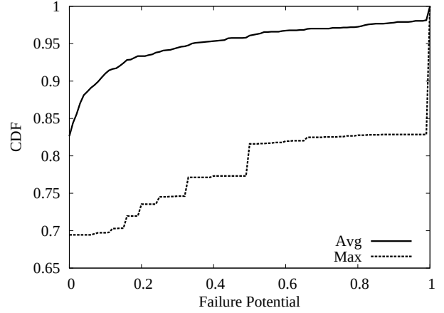
Fig. 4. The CDF describing the average and maximum failure potential for production signed zones during our analysis period.
