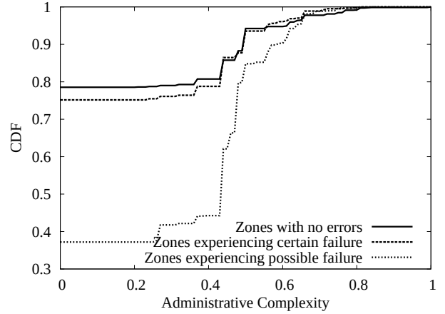
Fig. 5. The administrative complexity of production signed zones with no errors during our survey and those experiencing certain or possible validation failure.
