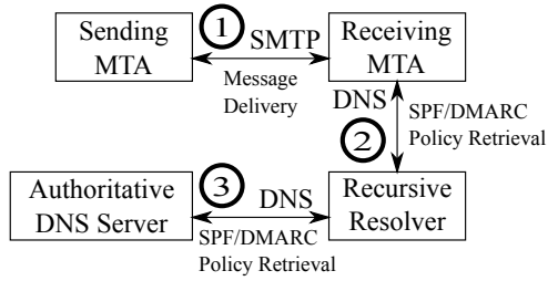
Figure 1: SPF policy retrieval using the DNS (2 and 3), in conjunction with SMTP message delivery (1).
