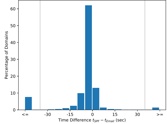
Figure 2: Distribution of the difference in timestamp between when the DNS query for an SPF policy was received ( t_{SPF} ) and when the corresponding email message was delivered ( t_{Email} ) in the NotifyEmail experiment.
